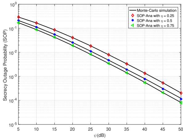
Fig. 4: The SOP versus \psi (dB) with varying \eta and R_{th} = 0.1 , \alpha = 0.5
