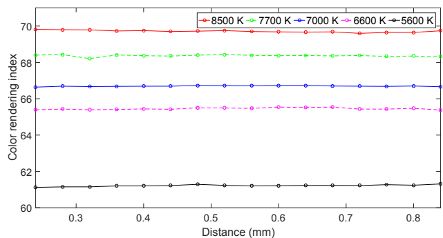
Fig. 5: The color rendering index of WLEDs as a function of d .
